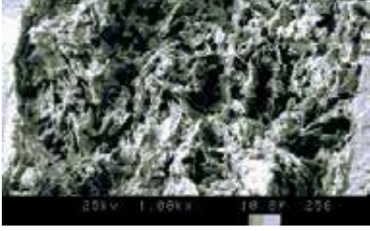
● Picture taken at 1,000x magnification using a SEM to demonstrate the fibrous nature of the FlexiCap™ termination that absorbs increased levels of mechanical stress.
