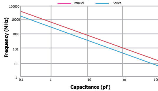
Resonant Frequency vs. Capacitance DLI C17 UL Series
