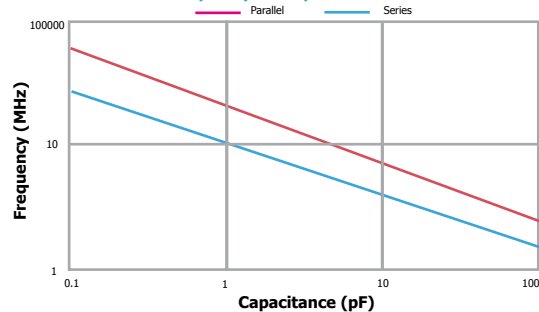
Resonant Frequency vs. Capacitance DLI C11 UL Series
