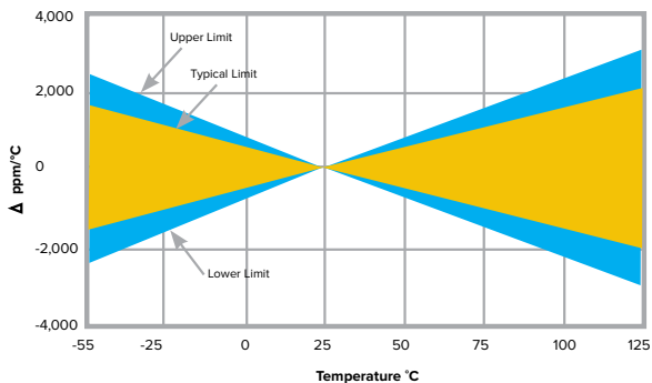
X7R (2R1)
