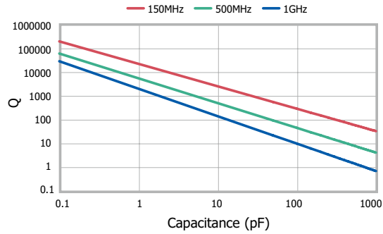
Q vs. Capacitance DLI C18 AH Series
