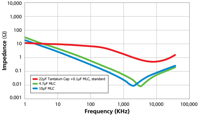
Impedance Curves
