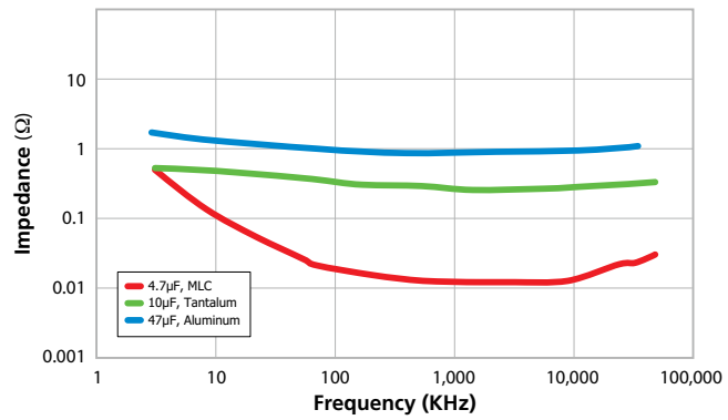
ESR Characteristics
