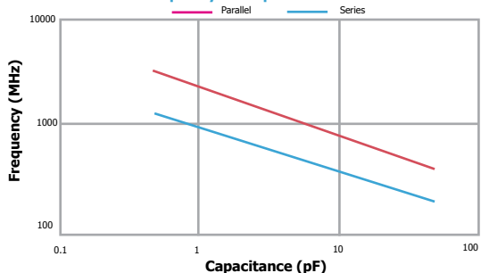
Resonant Frequency vs. Capacitance DLI C07 UL Series
