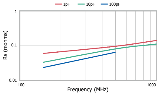
ESR vs. Frequency DLI C18 AH Series
