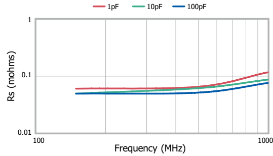
ESR vs. Frequency DLI C17 AH Series
