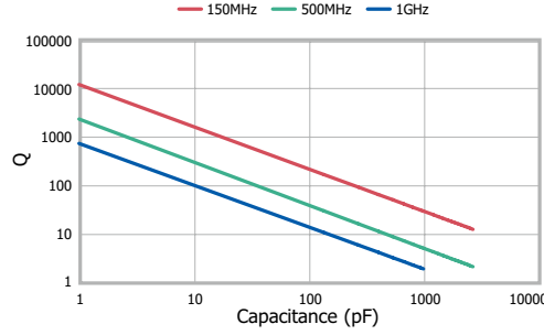
Q vs. Capacitance DLI C22 CF Series
